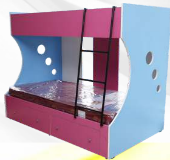
KIDS BUNKER COT SIZE(WxDxH) : 42x72x66
