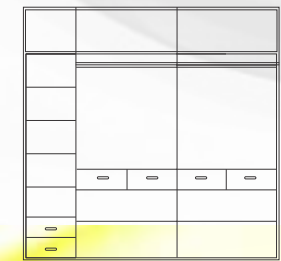
5 DOOR+INSIDE LOFT SIZE(WxDxH): 90x21x96
