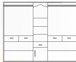
5 DOOR DRESSING SIZE(WxDxH): 90x21x78
